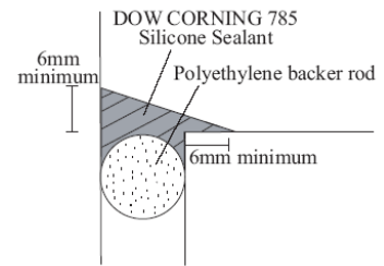
Figure 1: Fillet Joint.
