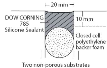
Figure 2: Deep joint.
