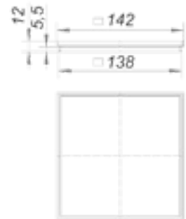
extension frame (480811)
