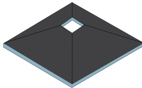
800 x 800 x 30mm Corner Drain
