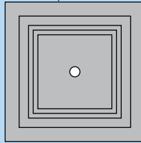
1500, 1200, 1000, 900 and 800 square centre drain
